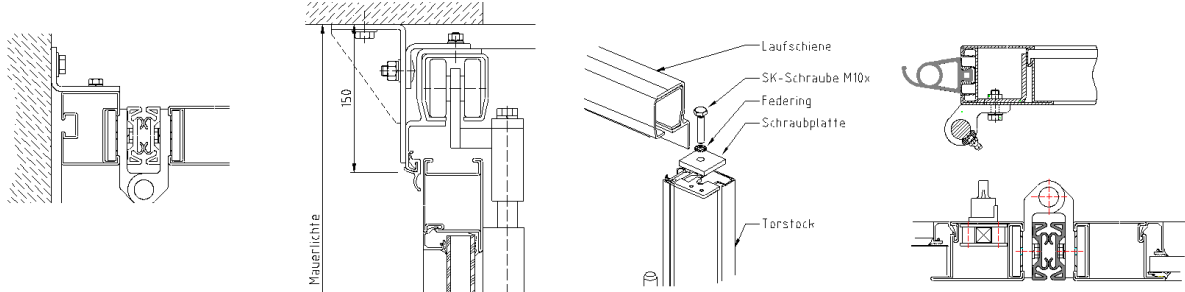
Running rail bolted connection
